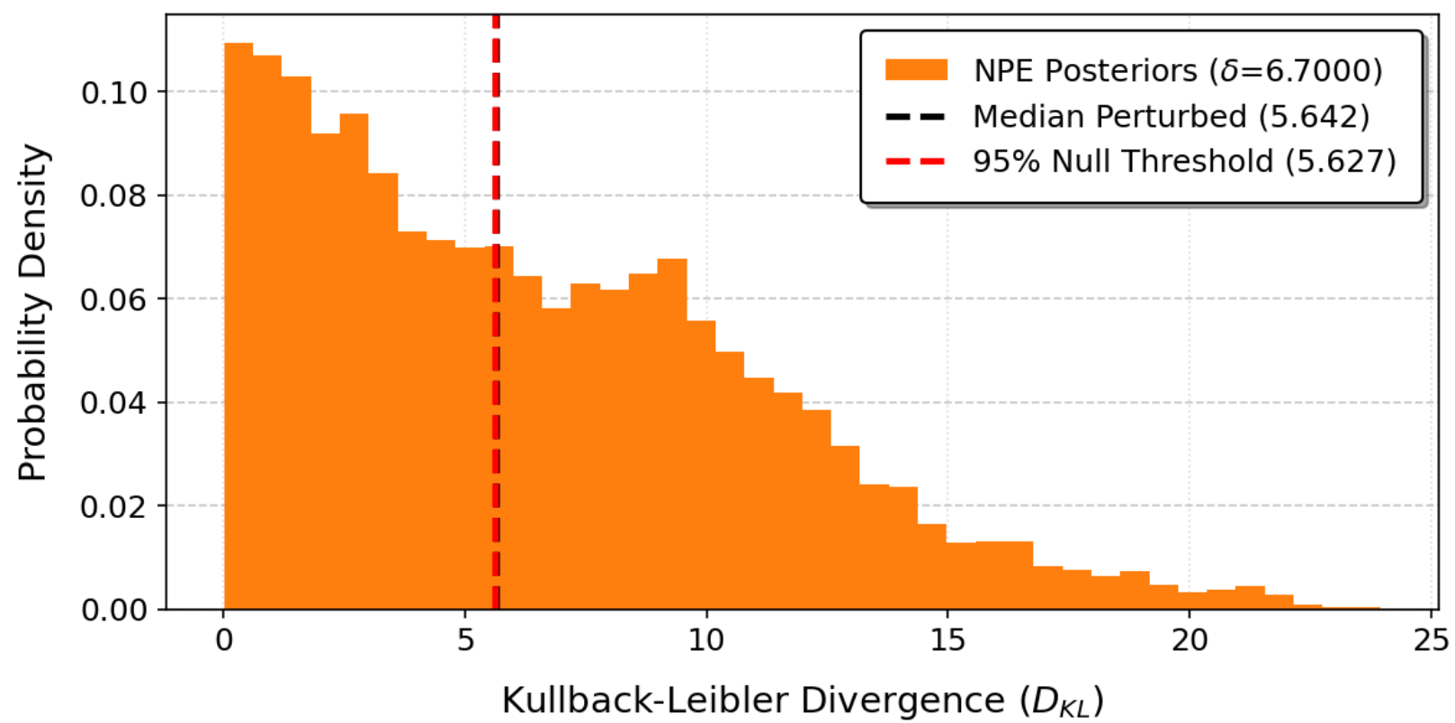
Perturbed D_{KL} -- \delta = 6.7000
